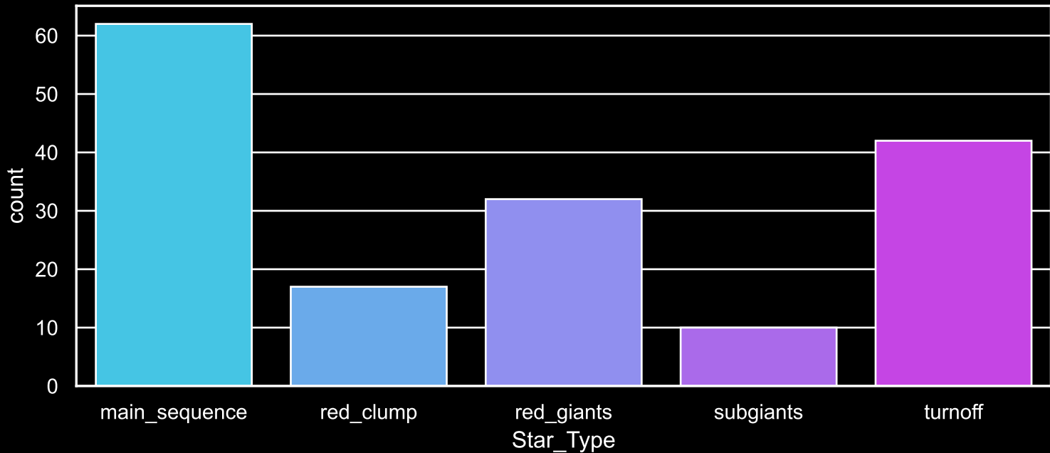
Field [42] Count plot of Star Type
