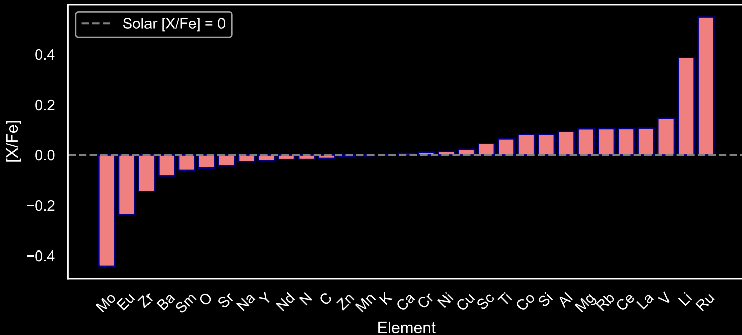
Abundance Pattern for GALAH Main Sequence Stars: Star Field [42] (N=62)
