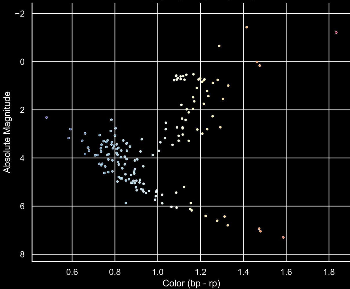
GALAH Hertzprung-Russel Diagram Field [42] Ra [325.64] Dec [-57.99]
