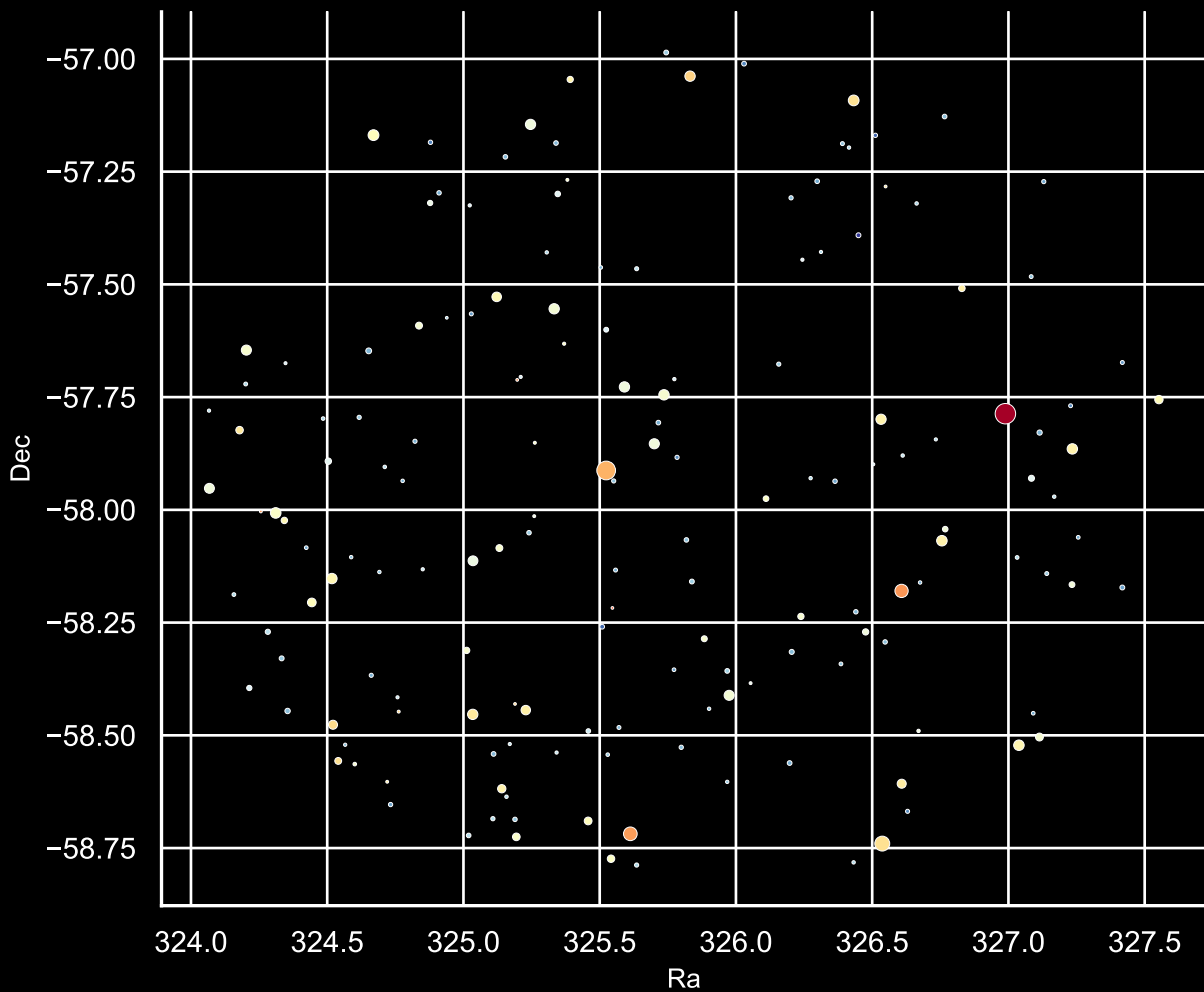
Field [42] Ra [325.64] Dec [-57.99] Stars: 163
